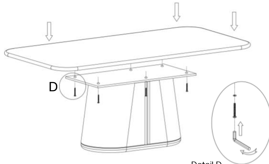
Detail D
